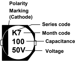
Fig.1 ΦD=4~ 10mm
