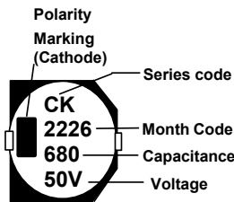
Fig.2 ΦD≥12.5mm
